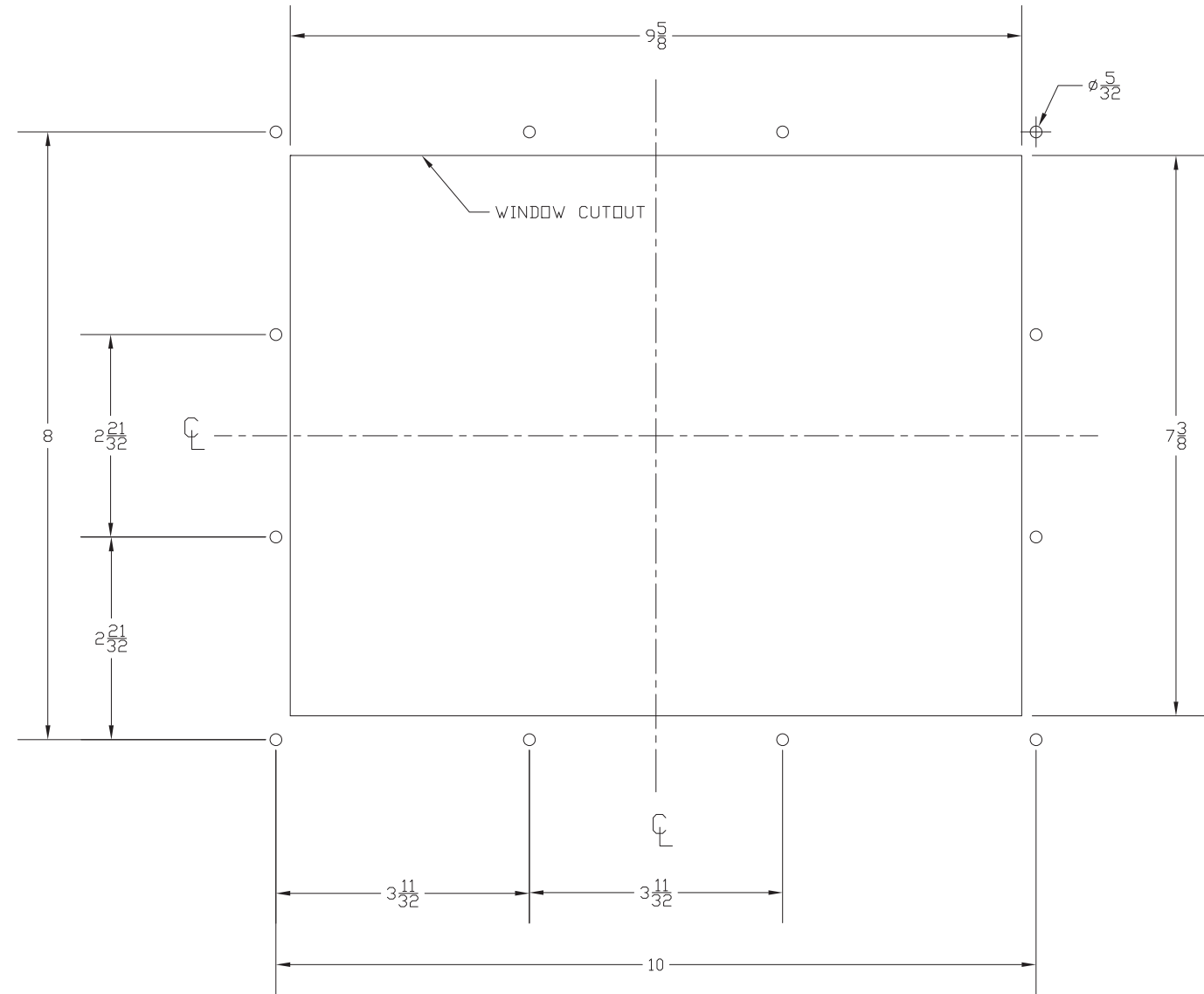
MOUNTING DETAIL
