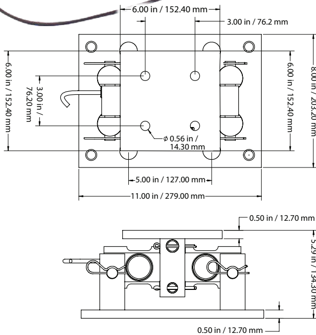
DB-20000SP / DB-20000SPS
