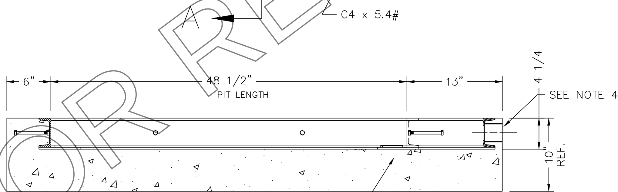
SECTION B-B
